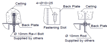
(Fastening Details)
