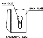
(FASTENING DETAILS)
