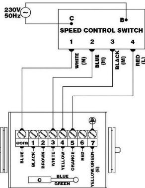
ELECTRO MOTOR WIRING DIAGRAM WITH SPEED 3-4-5
