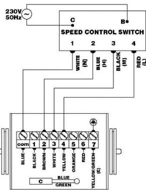
ELECTRO MOTOR WIRING DIAGRAM WITH SPEED 2-3-4
